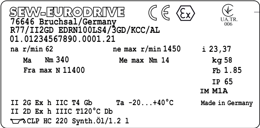
Nameplate
