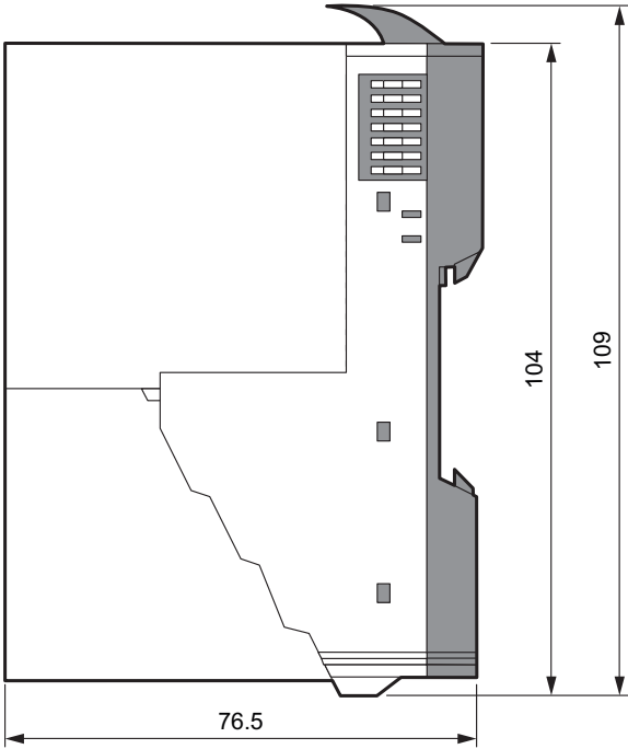
Bus coupler
