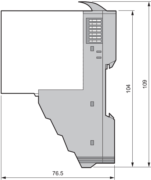
Peripheral module
