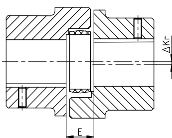
radial displacements
