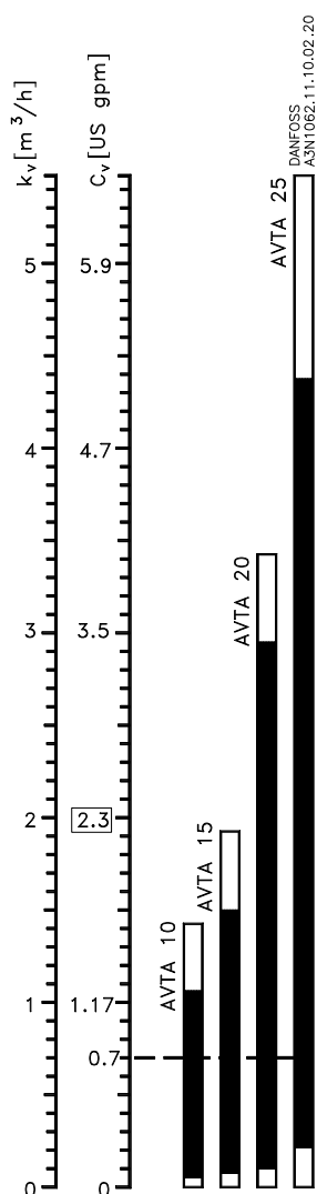
Fig. 1 Heating or cooling with water. Example: Necessary cooling output 10 kW with \Delta t = 10^\circ\text{C} Required flow 0.85 m³/h.
