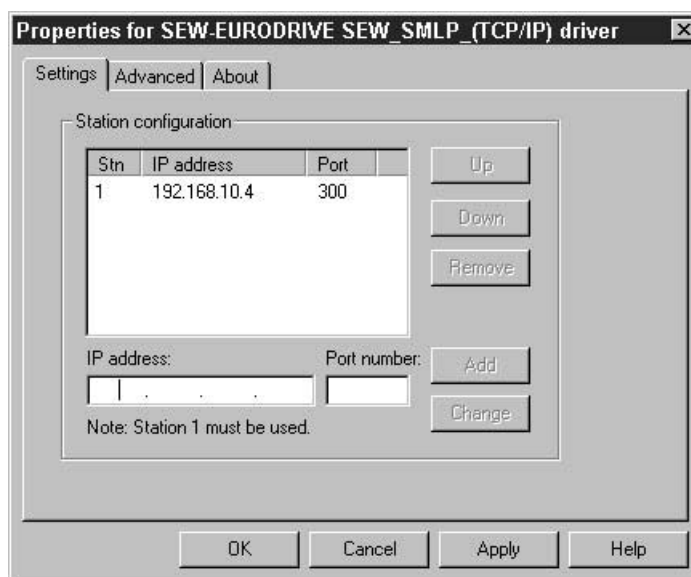
Рис. 26. Driver configuration
