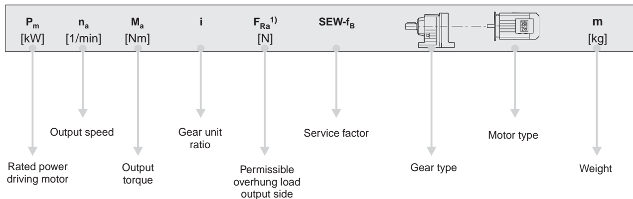
Fig. 1: Structure of the selection tables for R, F, K and S multi-speed geared motors
