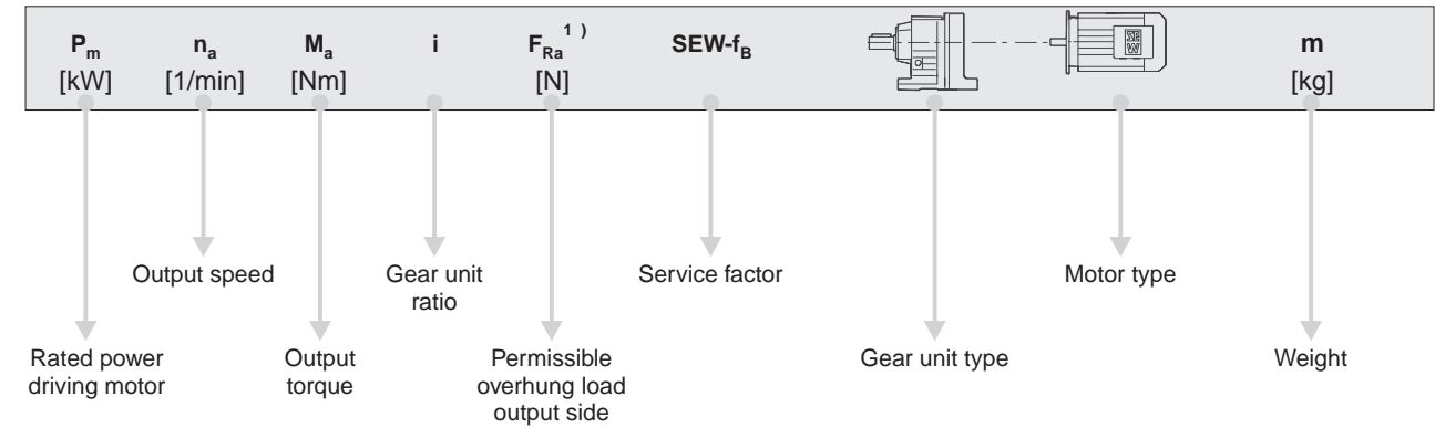
Fig. 2: Structure of the selection tables for W multi-speed geared motors
