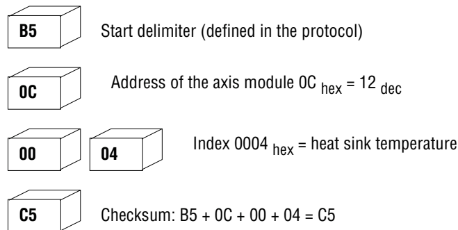
Figure 10: Sending the ENQUIRY frame
