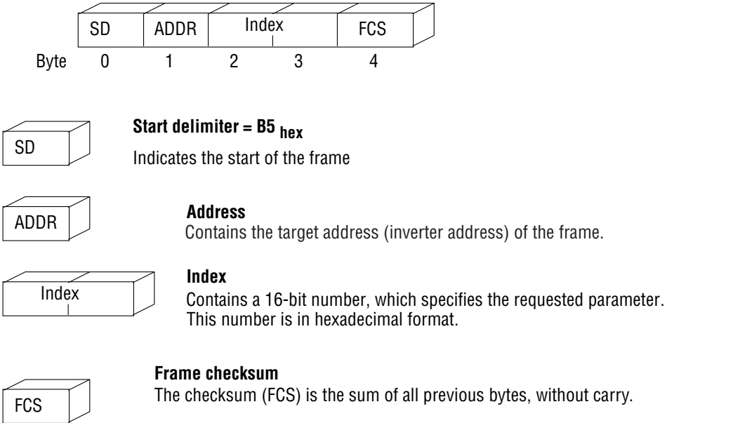
Figure 3: ENQUIRY frame
