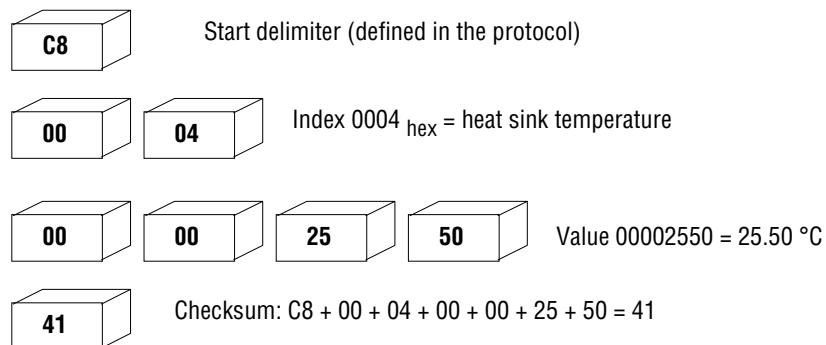
Figure 11: Replying with a DATA frame
