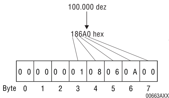
Figure 23: 8-byte format
