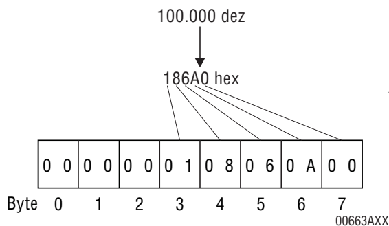
Figure 23: 8-byte format
