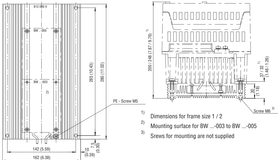
Fig. 1: FKB01 Heat sink for brake resistors in flatpack design, dimensions in mm (in)
